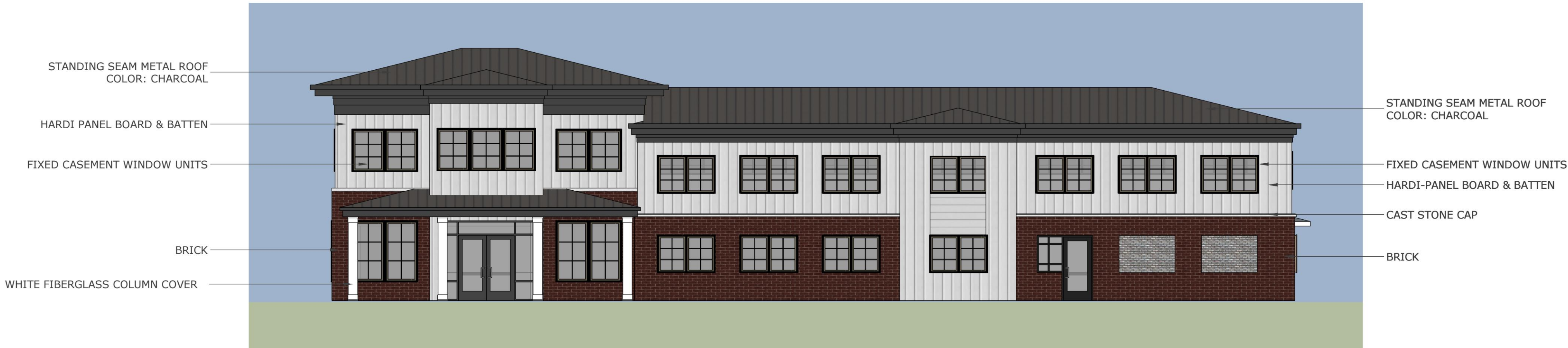
FRONT ELEVATION
